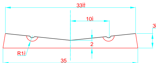
TRANSVERSAL SECTION "A" SECCION TRANSVERSAL "A"
