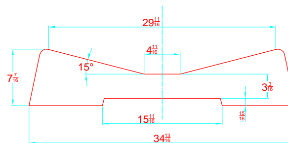
TRANSVERSAL SECTION "A" SECCION TRANSVERSAL "A"
