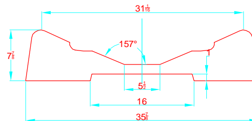
TRANSVERSAL SECTION "A" SECCION TRANSVERSAL "A"
