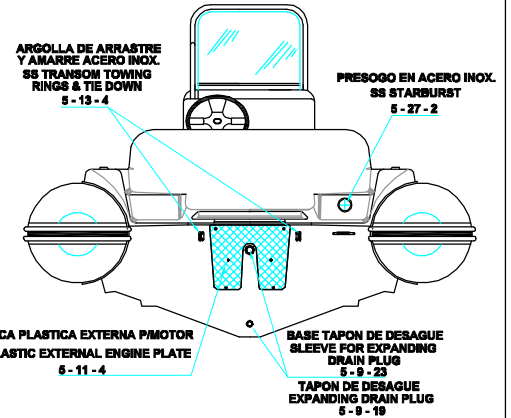
AFT VIEW VISTA TRASERA
