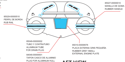
AFT VIEW
