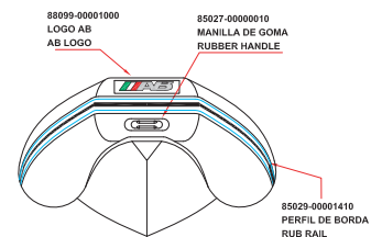
FORE VIEW
