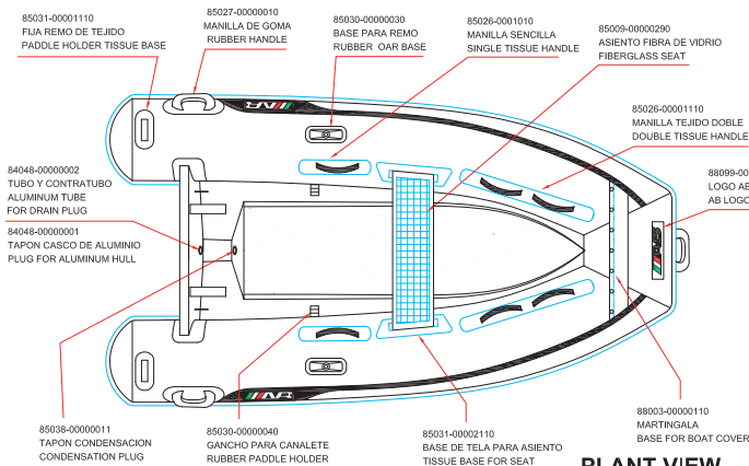
PLANT VIEW
