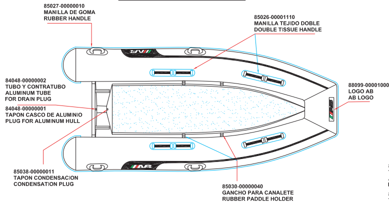
PLANT VIEW
