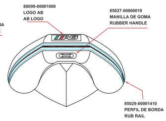
FORE VIEW
