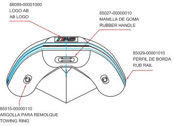
FORE VIEW
