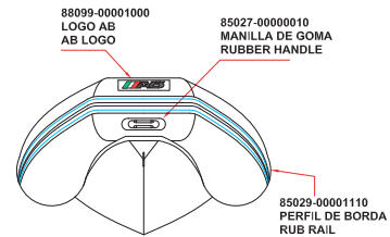
FORE VIEW
