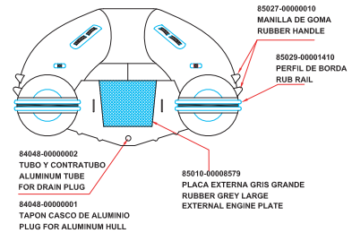
AFT VIEW
