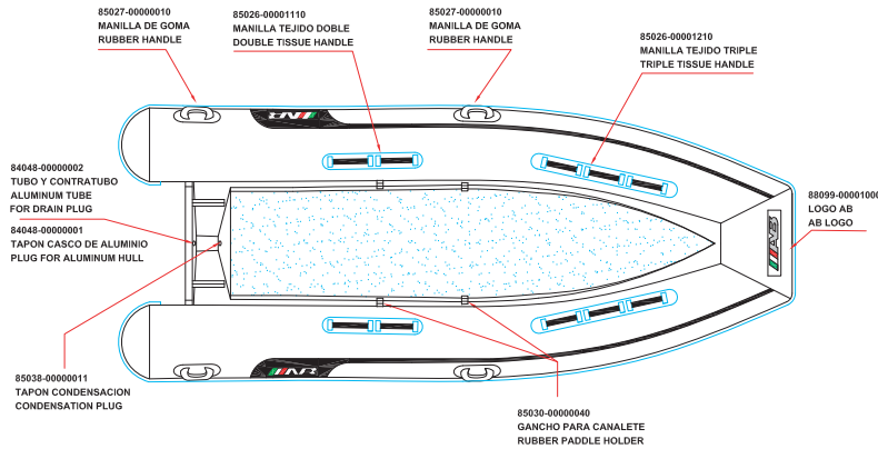
PLANT VIEW
