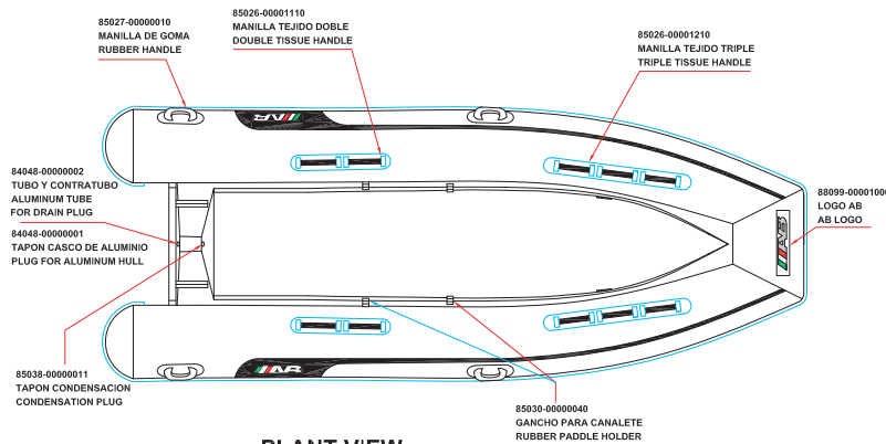
PLANT VIEW
