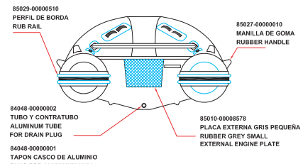
AFT VIEW
