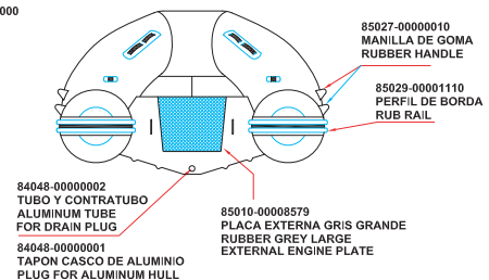
AFT VIEW
