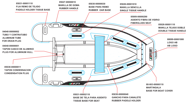
PLANT VIEW
