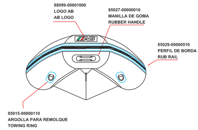
FORE VIEW
