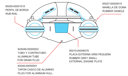
AFT VIEW
