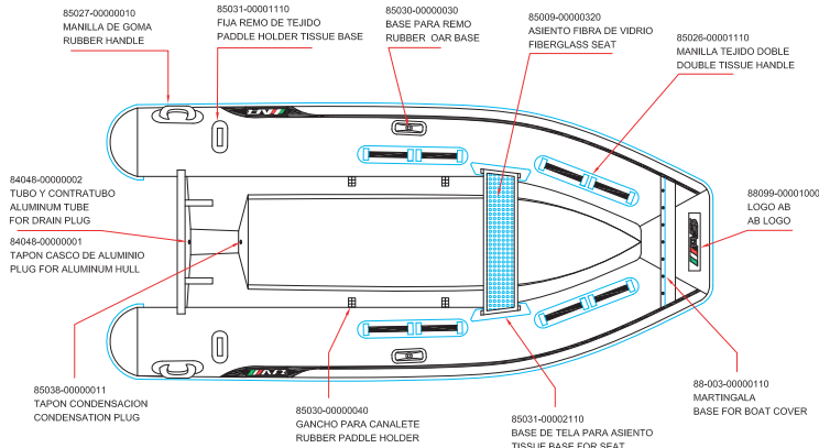
PLANT VIEW
