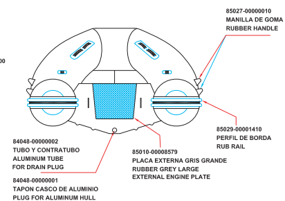
AFT VIEW
