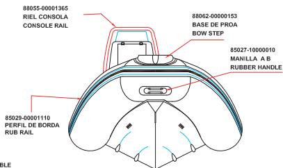
FORE VIEW
