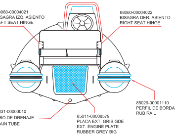
AFT VIEW
