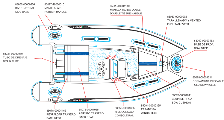
PLANT VIEW
