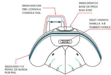
FORE VIEW
