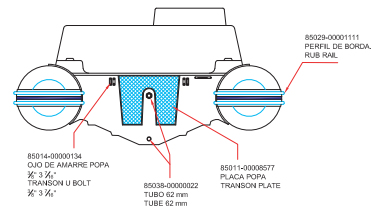
AFT VIEW
