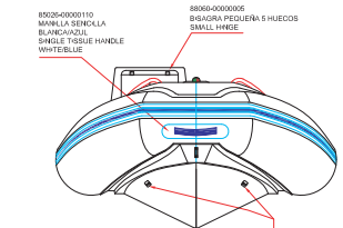
AFT VIEW
