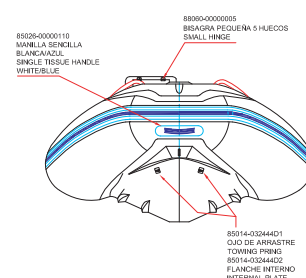
FORE VIEW
