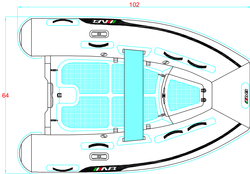
PLANT VIEW VISTA SUPERIOR
